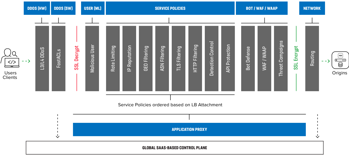
Figure 4: Logical flow of client app requests through F5 Distributed Cloud WAAP security functions
