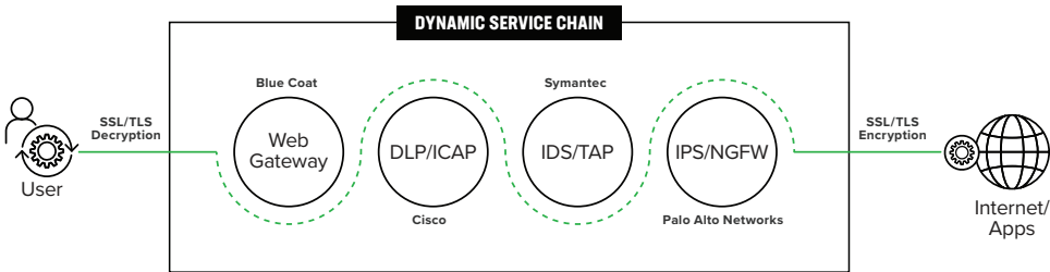
Figure 2: BIG-IP SSL Orchestrator enables the creation of dynamic service chains based on traffic classification.
